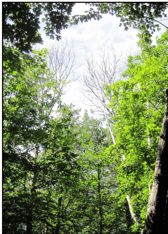
Succession in progress: small-scale age-related mortality at UMBS, with two dead aspens standing over a proliferating maple subcanopy.
