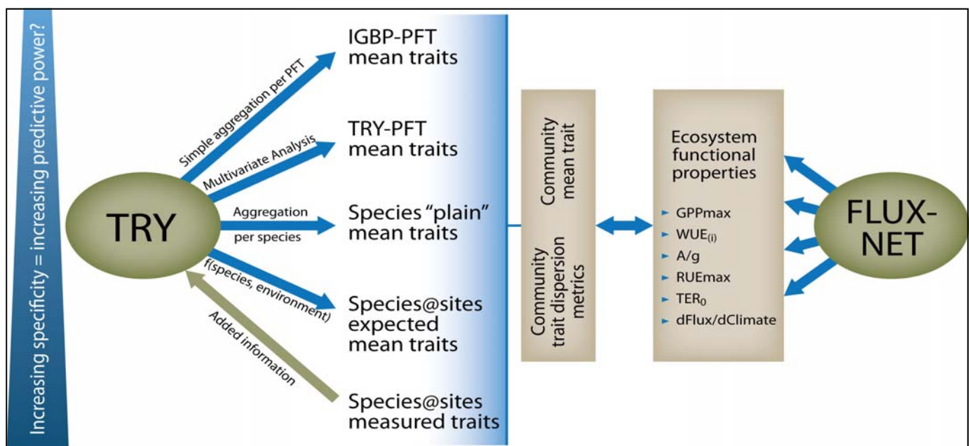
Figure 3: Schematic approach to disentangle the impact of plant traits on ecosystem functional properties by a stepwise adding of specific trait information. Developed at the TRY workshop 2011 (M. Reichstein/M. Bahn).
